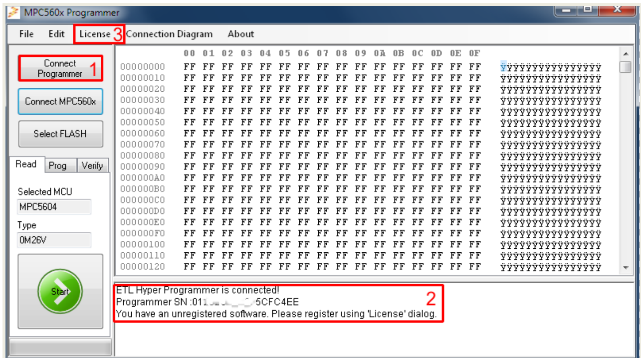
Figure 19 MPC560x-Programmer software
