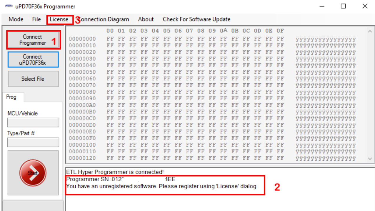
Figure 19 UPD70F36x-Programmer software
